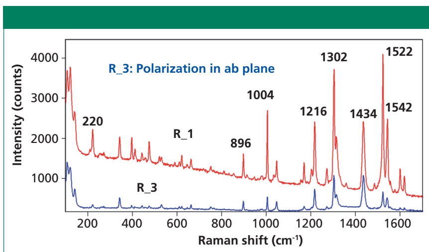
Figure 8: Raman spectra of different grains of rubrene.
