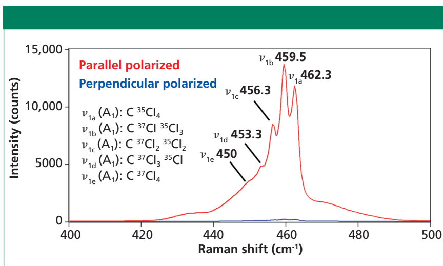
Figure 3: A 1 Symmetric stretching band of CCl 4 . The band is split in accordance with the isotopic abundance of Cl.
