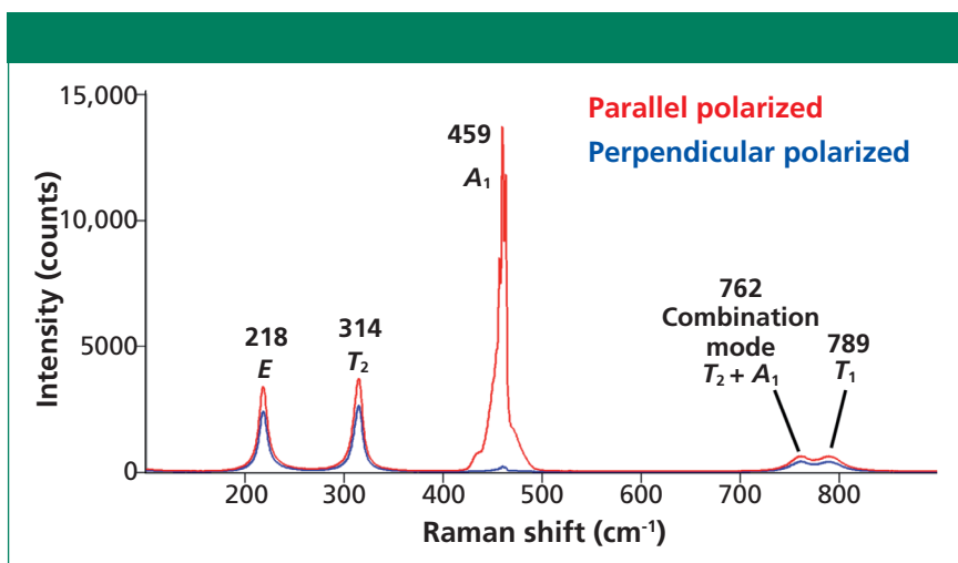
Figure 2: Polarized Raman spectra of CCl 4 .
