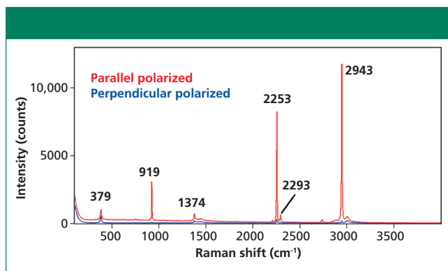
Figure 5: Polarized Raman spectra of acetonitrile.
