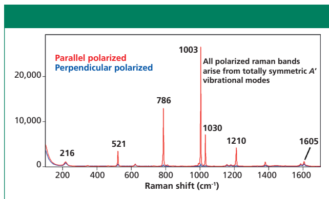
Figure 4: Polarized Raman spectra of toluene.
