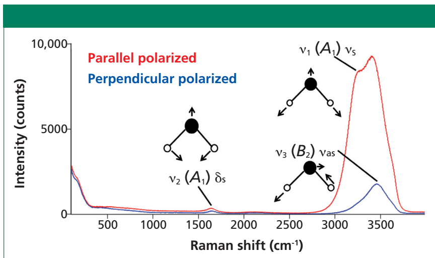
Figure 1: Polarized Raman spectra of H 2 O.
