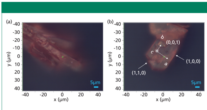
Figure 7: Reflected light images of rubrene grains (a) R_1 and (b) R_3.
