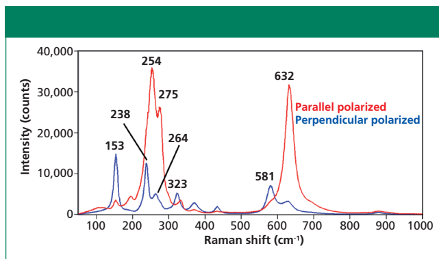
Figure 6: Polarized Raman spectra of the X -face of single crystal \text{LiNbO}_3 with the incident laser polarized along the Z -axis.
